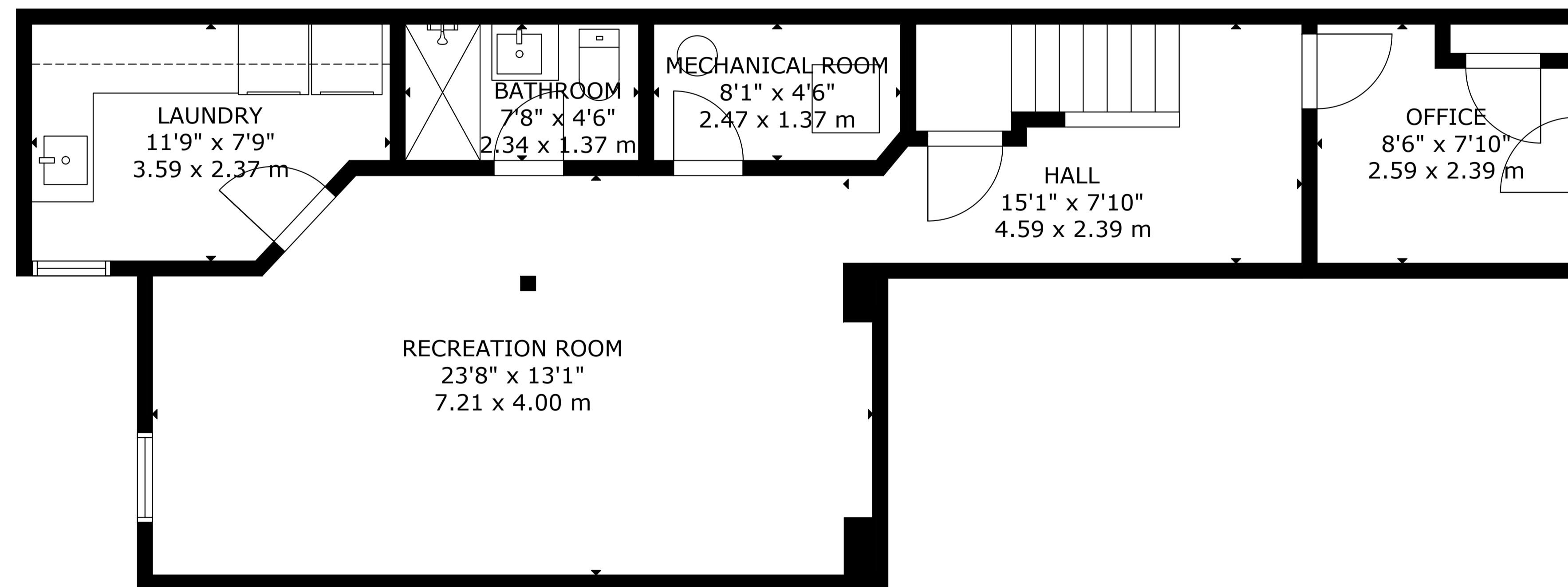
LOWER FLOOR
