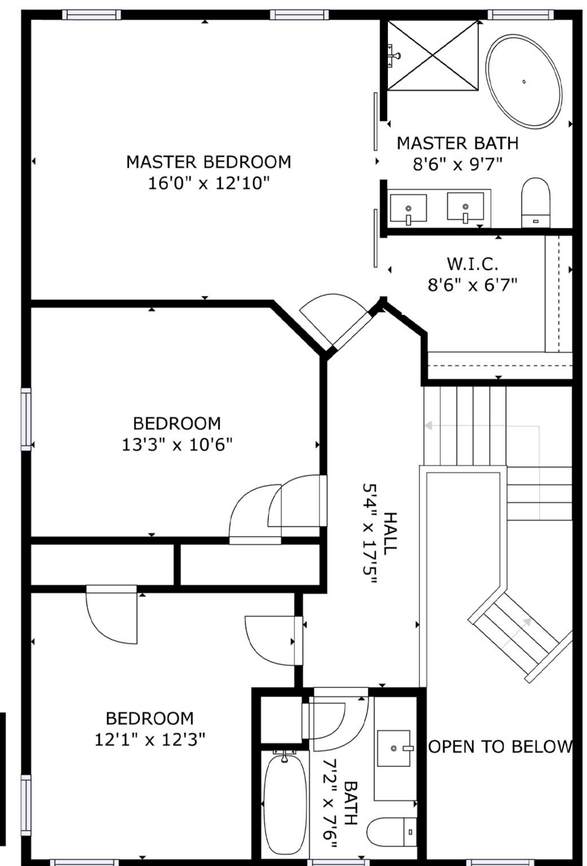
SECOND FLOOR
