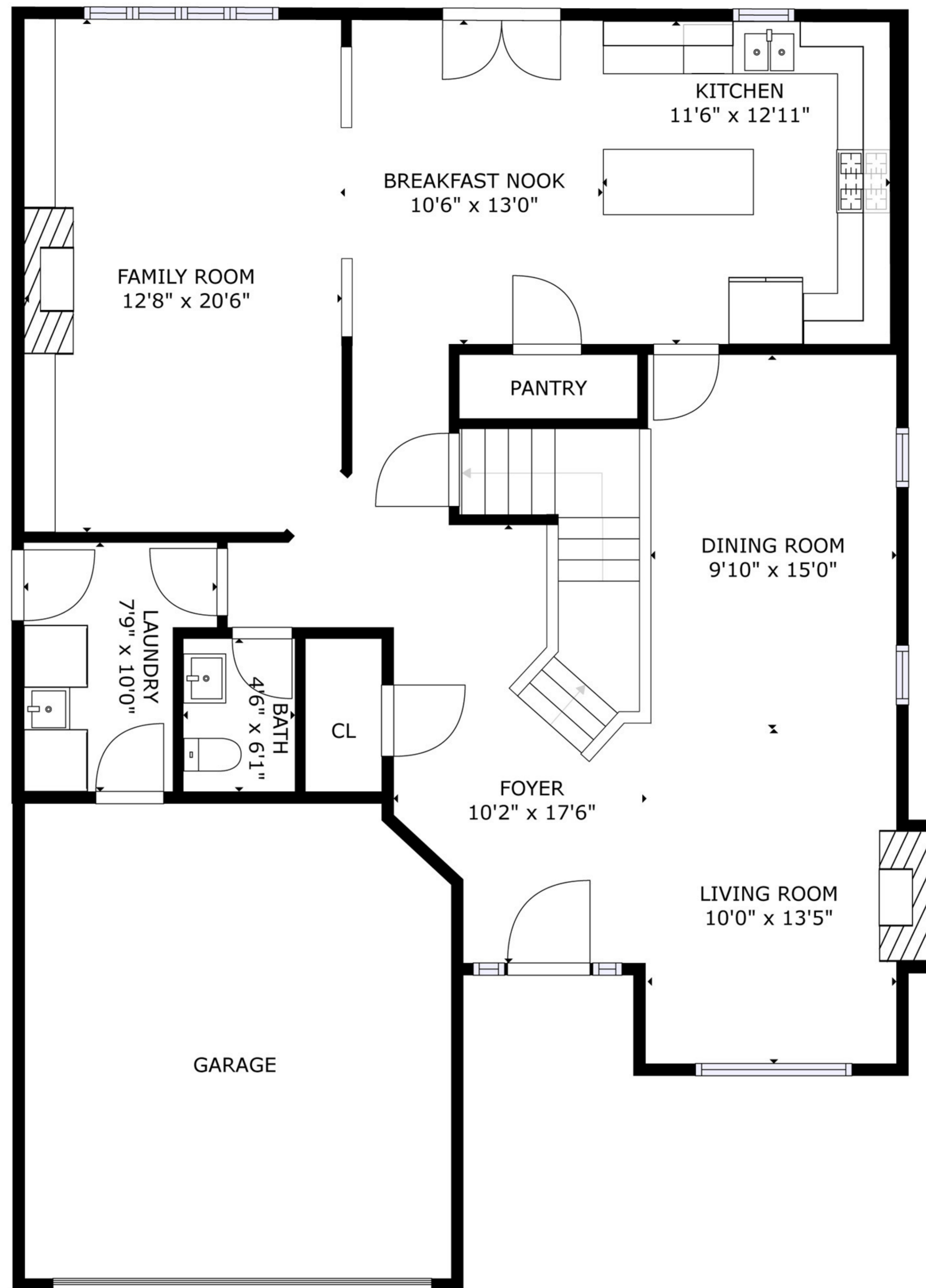
MAIN FLOOR
