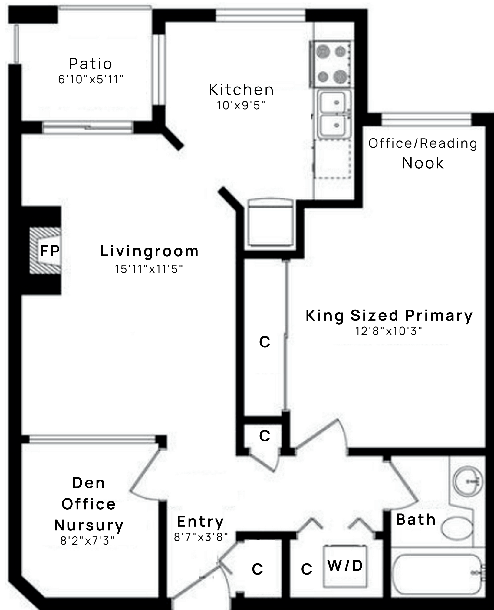
floor sketch overview - verify accuracy to your satisfaction
