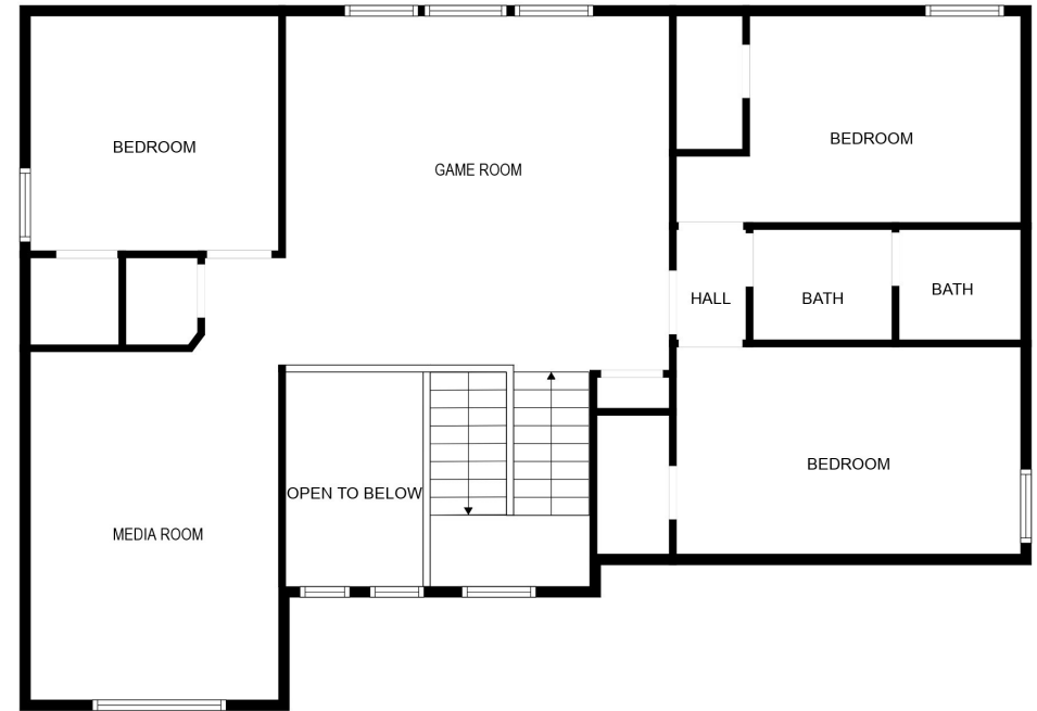
FLOOR 2
