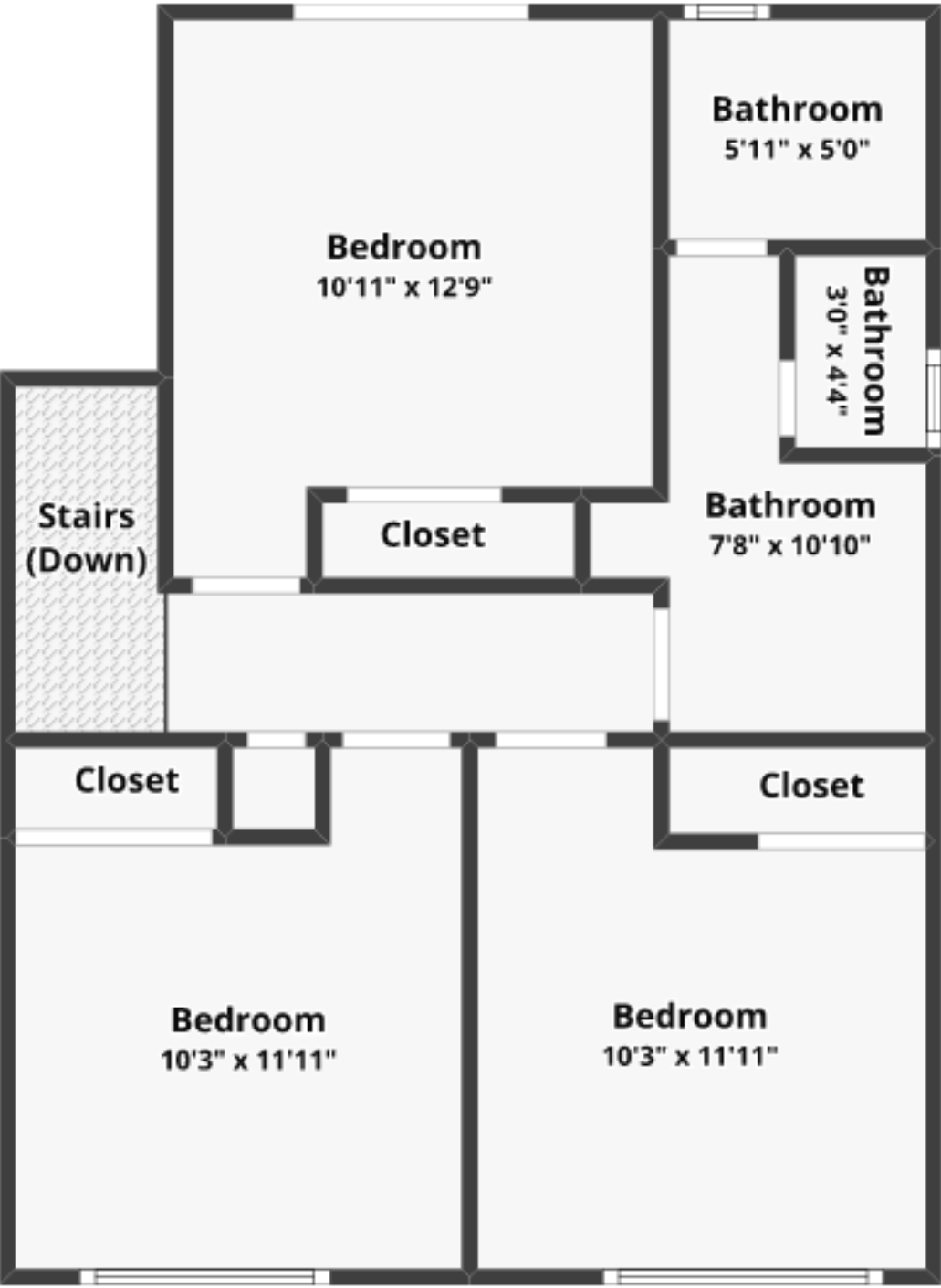
FLOOR 2
